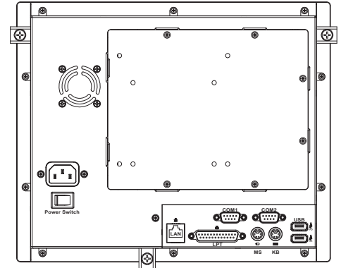
Rear View - with AC Socket
