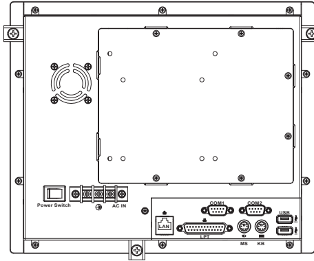
Rear View - with Terminal Block
